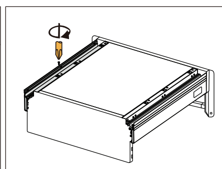
Base assembly
