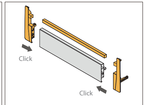
Front assembly
